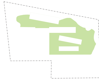
laag 1: gras
