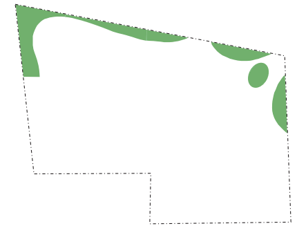
laag 3: heesters
